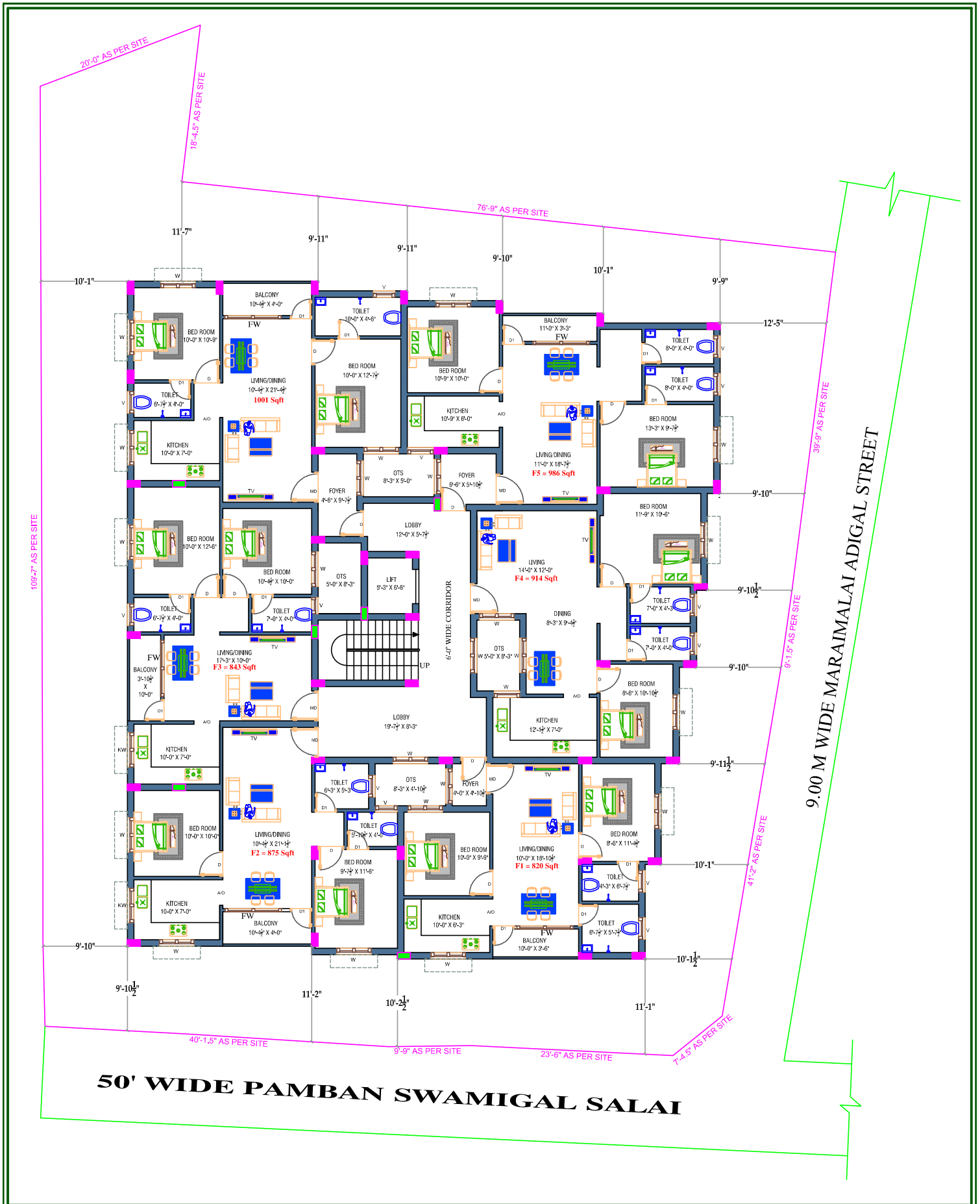
TYPICAL- 1st, 2nd ,3rd ,4th &5th FLOOR PLAN
